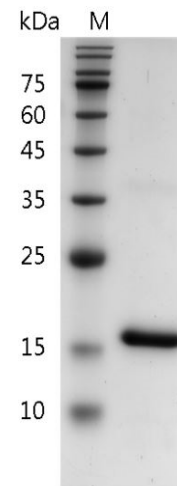
SDS-PAGE analysis of recombinant mouse IL-18
